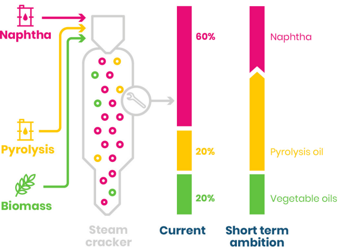
Figure 15 Mass balance
